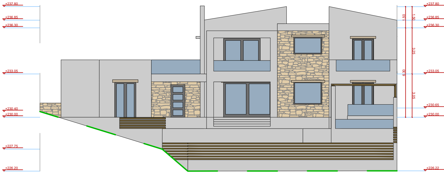
NORTHERN FACADE
